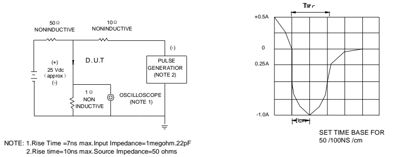
FIG.6-TEST CIRCUIT DIAGRAM AND REVERSE RECOVERY TIME CHARACTERISTIC
