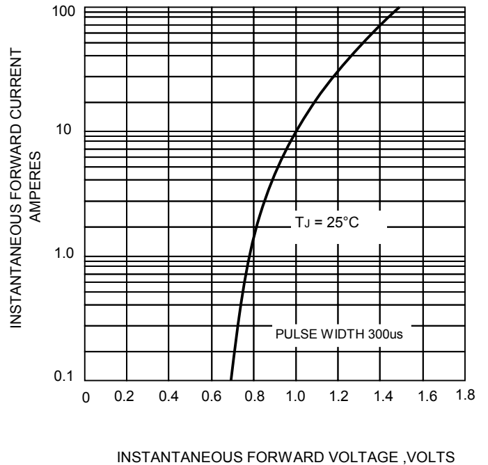
FIG.4-TYPICAL FORWARD CHARACTERISTICS
